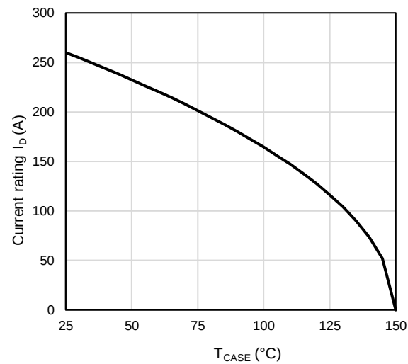
Figure 12: Current De-rating
